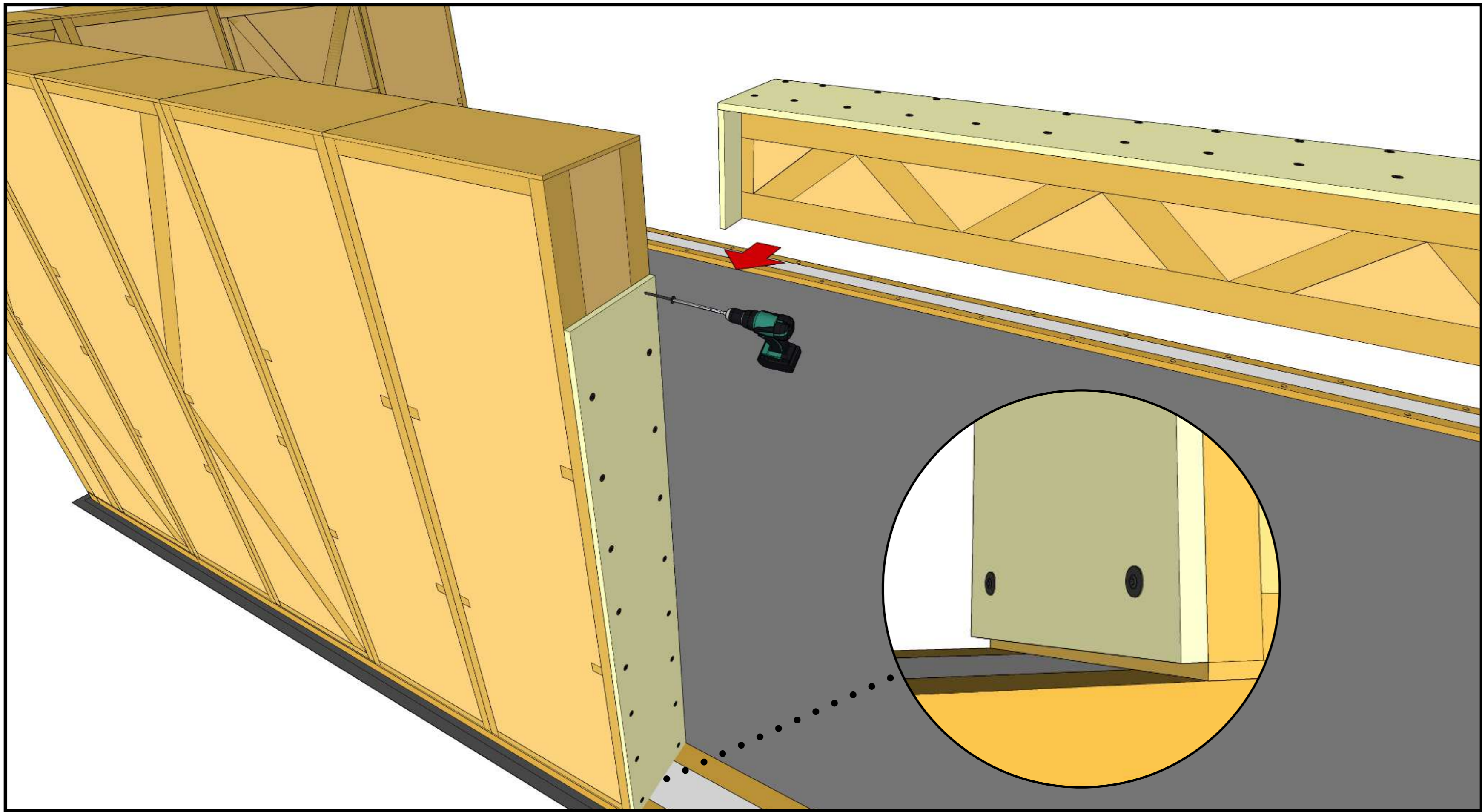
Fix the plywood boards for the window reveal tight to the lintel. Leave a small (approximately 3/32 inches) gap at the bottom.
