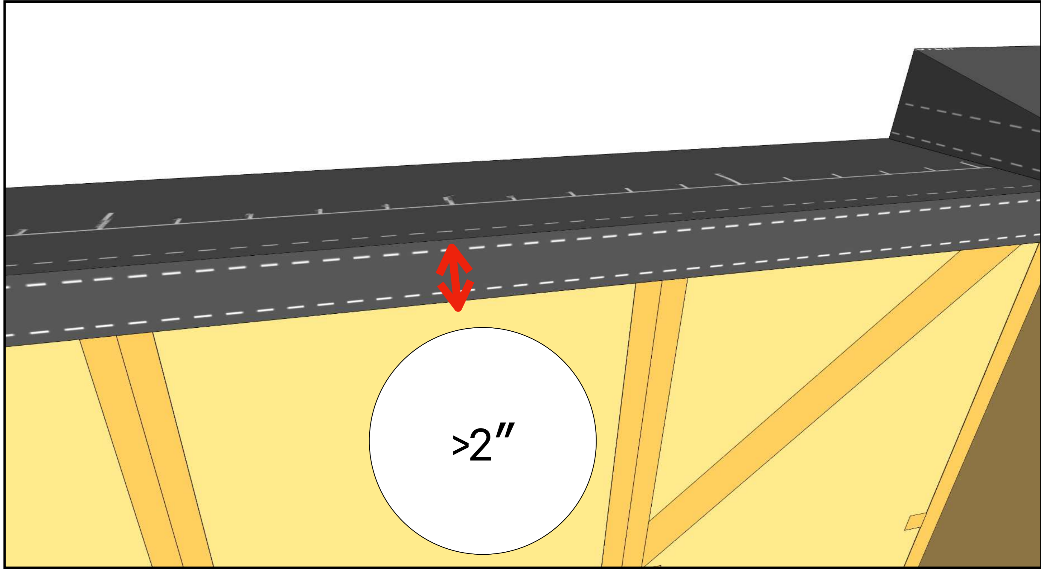
Flip the membrane over the top and leave 2 inches projecting to the interior side. If you pause work overnight, ensure the top is covered with a strip of membrane.
