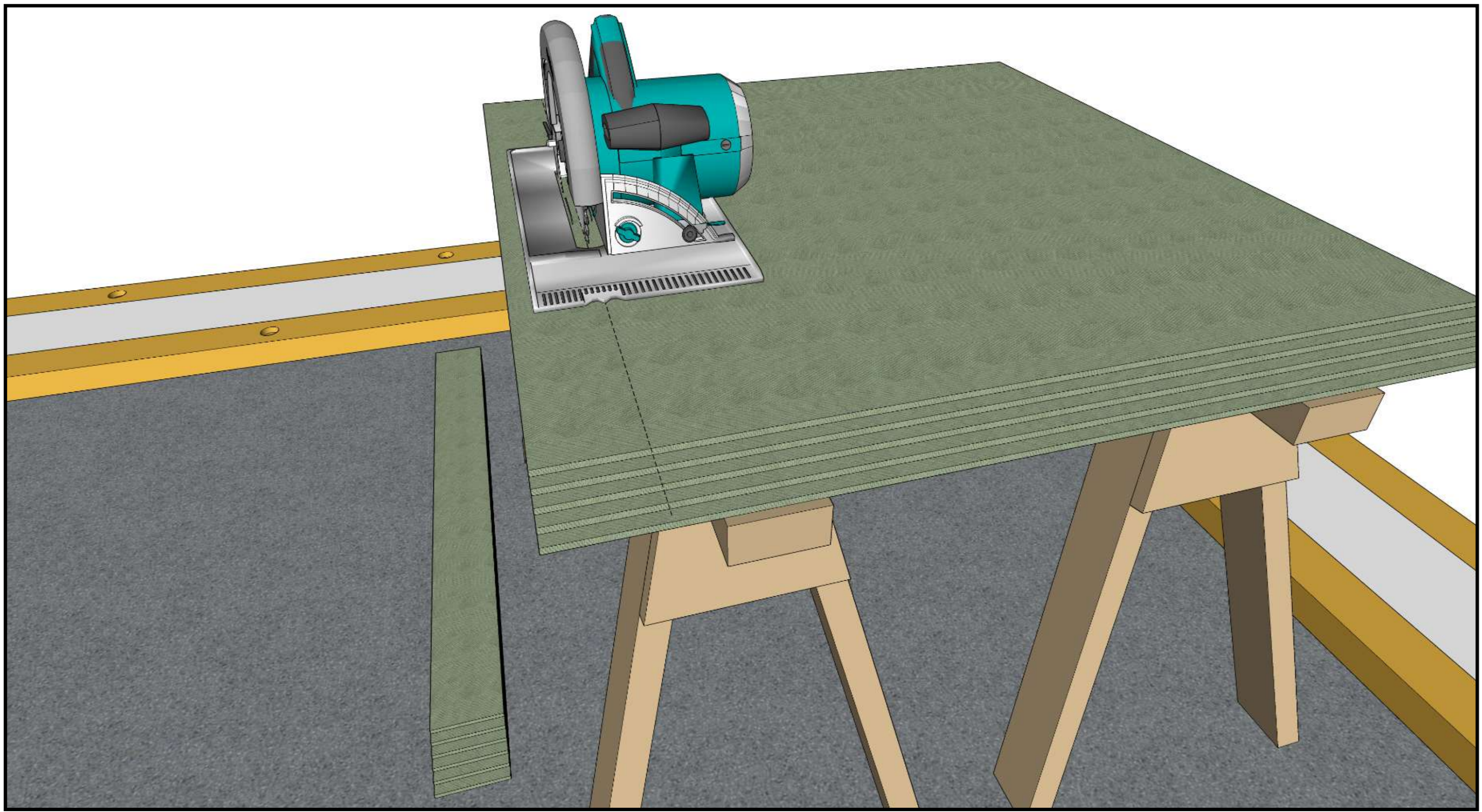
Cut 1/4 inches thick wood fibre board into strips to cover the timber structure.
