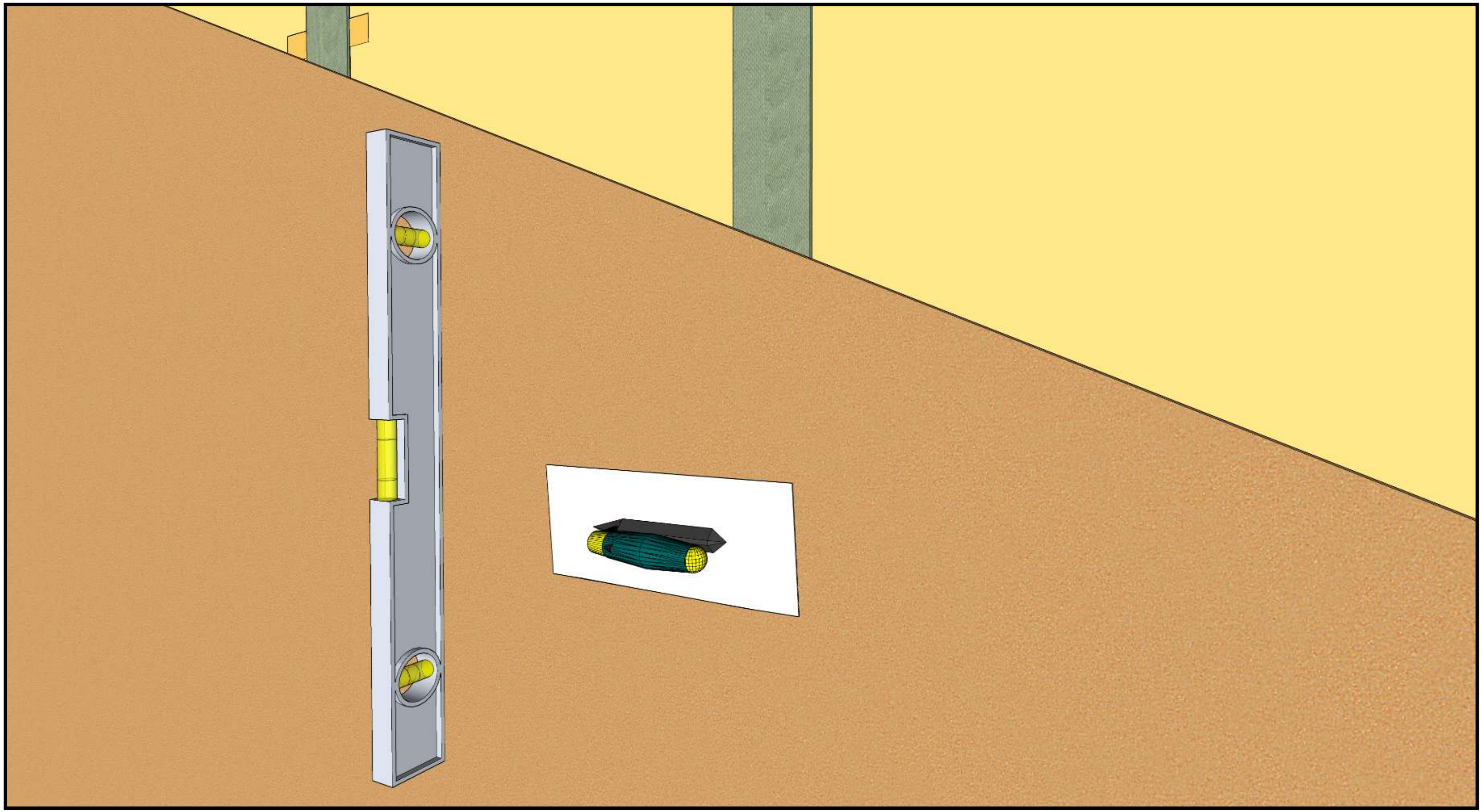
Apply the base coat plaster to a depth of 3/4 - 1 inches. This can be applied in one or two coats, with a reinforcing mesh either between 2 layers or into the top surface.
